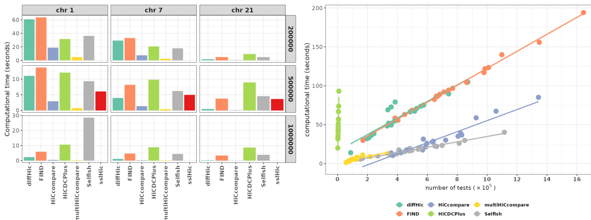
Fig. 8. Computational time. Left: Computational time in seconds ( y -axis) needed for each tool ( x -axis) to run in the H_1 setting. ssiHiC could only be used on 500 kb resolution data and multiHiCcompare performed no test on chromosome 21 because of its filtering step. Right: Computational time in seconds ( y -axis) versus the number of tests performed in a given chromosome ( x -axis) for the CTCF depletion dataset. ssiHiC could not be used.
